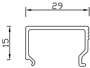
30971 Glazing Bead
