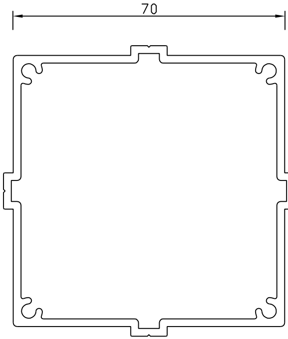
30976 Post
